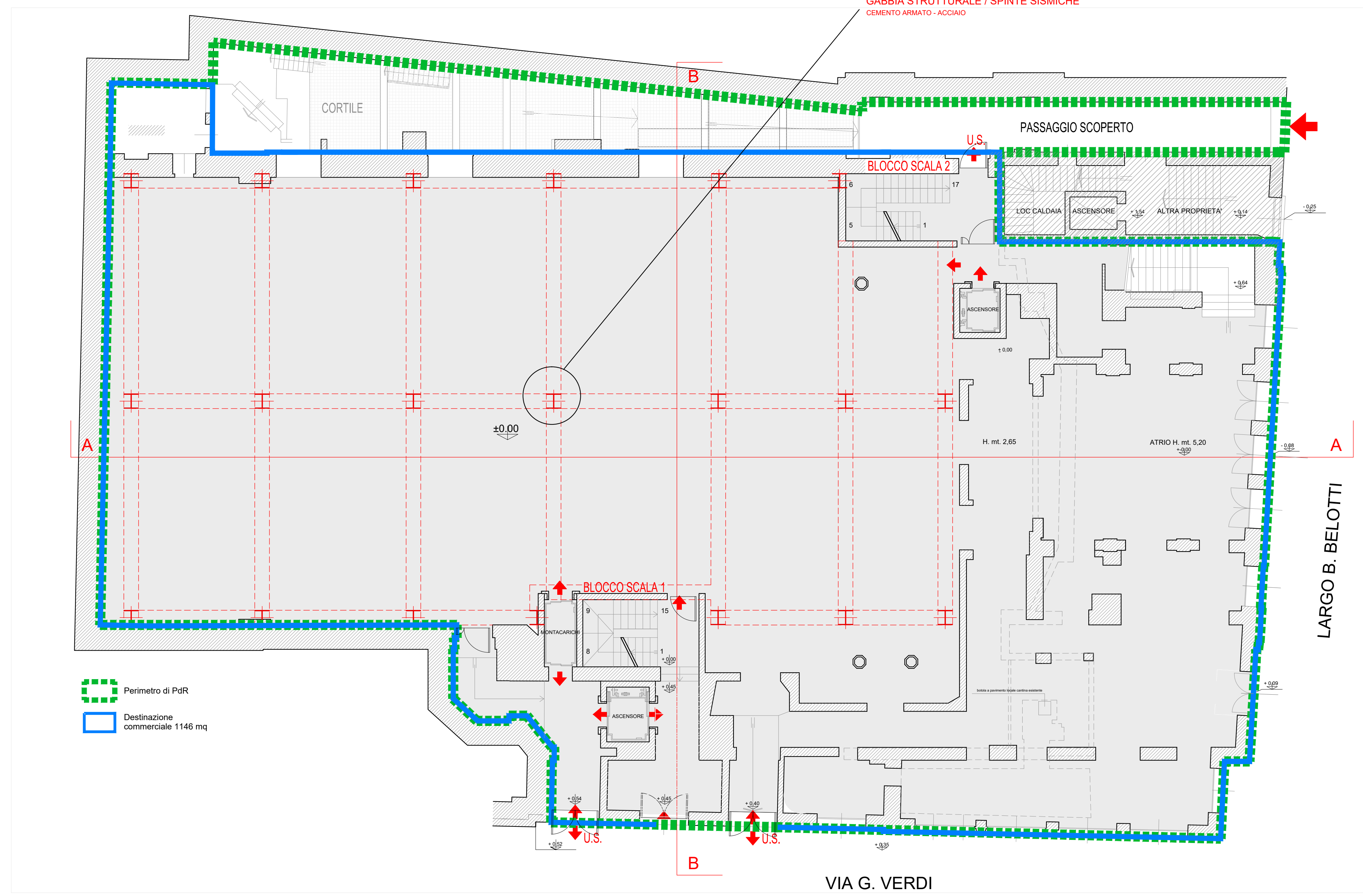
PLANIMETRIA PIANO TERRA
